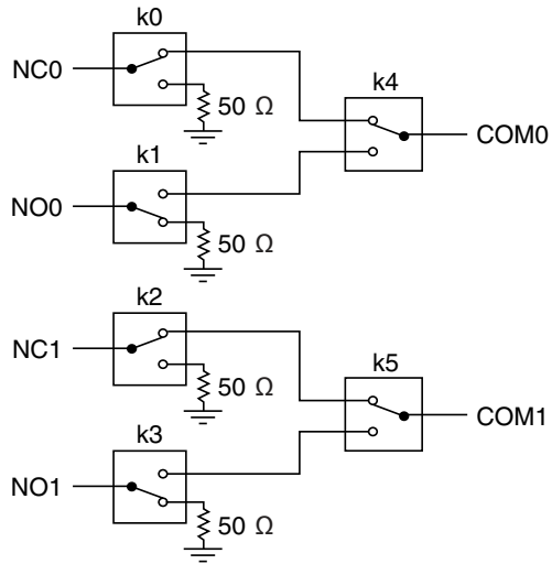
Figure 6. PXI-2549 Power-On State
