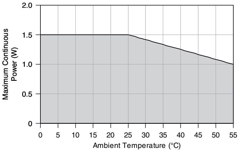
Figure 5. Termination Derating
